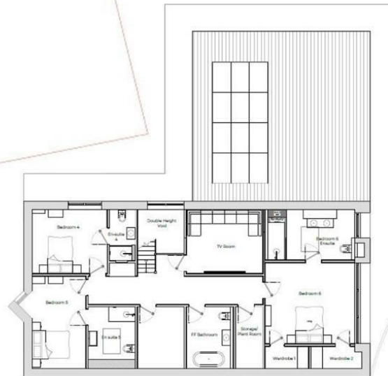
01 PROPOSED FF LAYOUT PLAN SCALE 1:50
